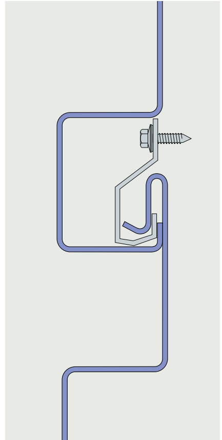
Panel Clip Detail
