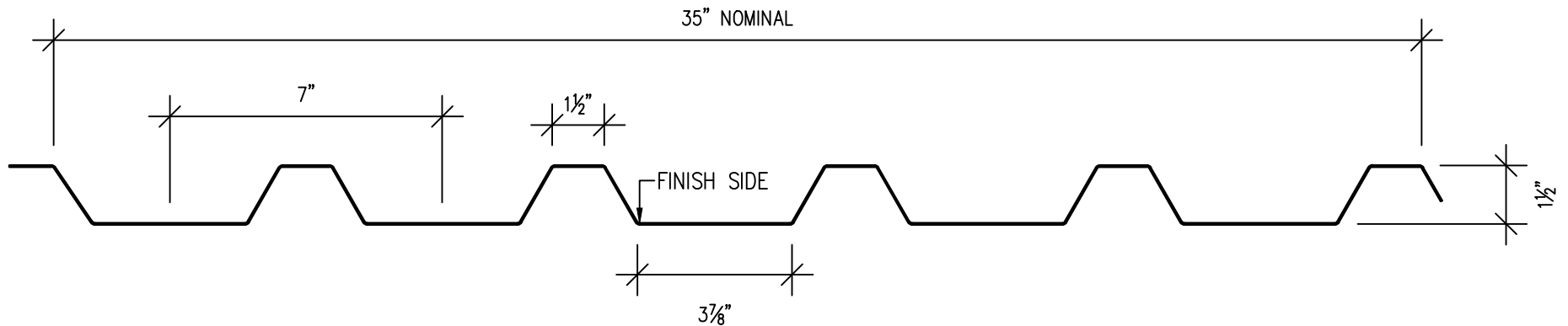
PROFILE A
