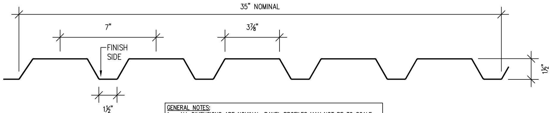
PROFILE B
