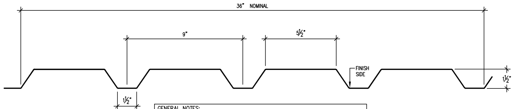
PROFILE B
