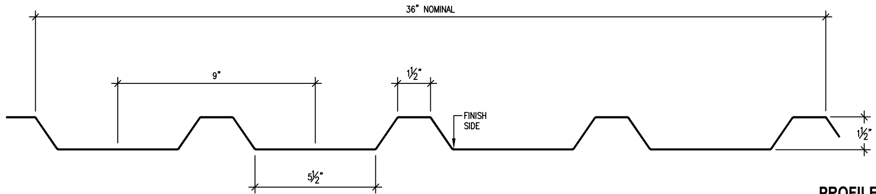
PROFILE A
