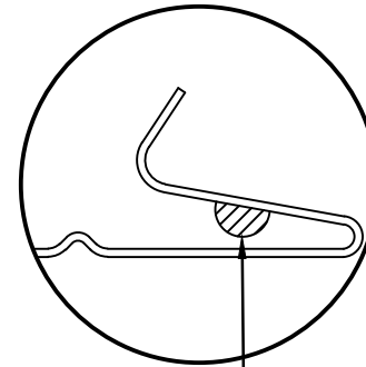
OPTIONAL FACTORY SEALANT (BUTYL PLACEMENT)
