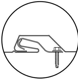
CLIP ENGAGEMENT
