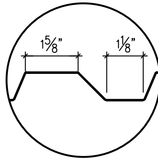
HIGH & LOW CELL DIMENSIONS
