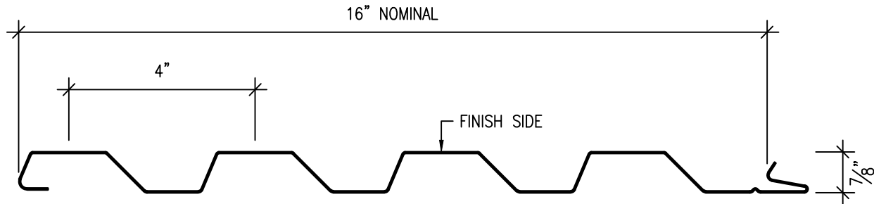
HIGH & LOW CELL DIMENSIONS
