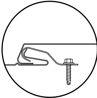
CLIP ENGAGEMENT
