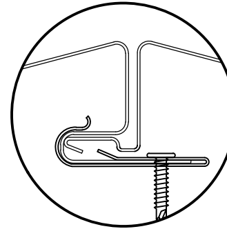
GENERAL CLIP ENGAGEMENT
