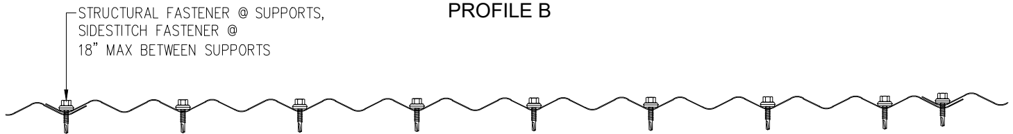
C-40-W FASTENING PATTERN PROFILE B
