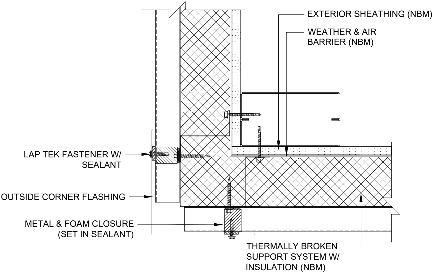
OUTSIDE CORNER DETAIL
