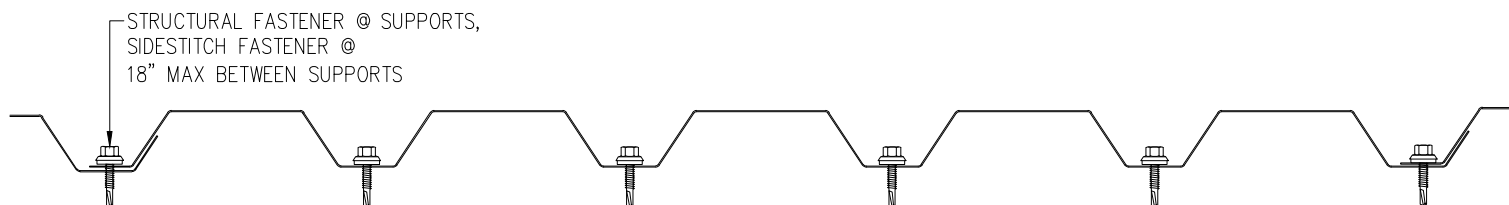
BR7-35-W FASTENING PATTERN PROFILE B
