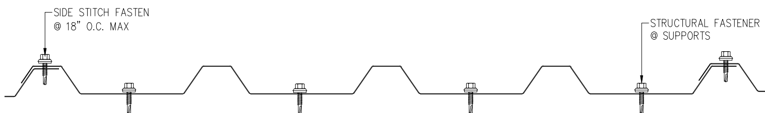
BR9-36-W FASTENING PATTERN PROFILE A
