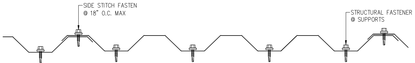
Y-29-ES FASTENING PATTERN PROFILE A
