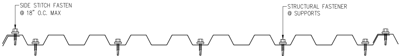
VB-36-W FASTENING PATTERN PROFILE A
