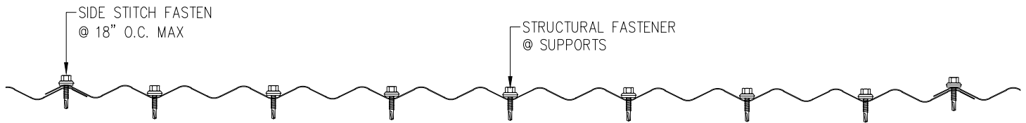
C-40-E FASTENING PATTERN PROFILE A
