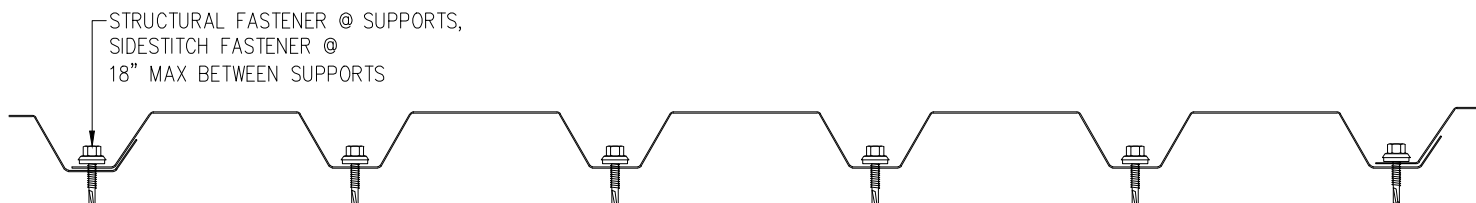
BR-35-S FASTENING PATTERN PROFILE B
