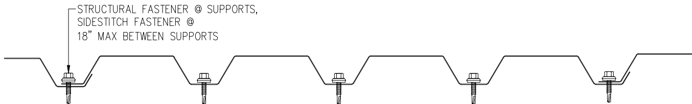
BR-28-ES FASTENING PATTERN PROFILE B
