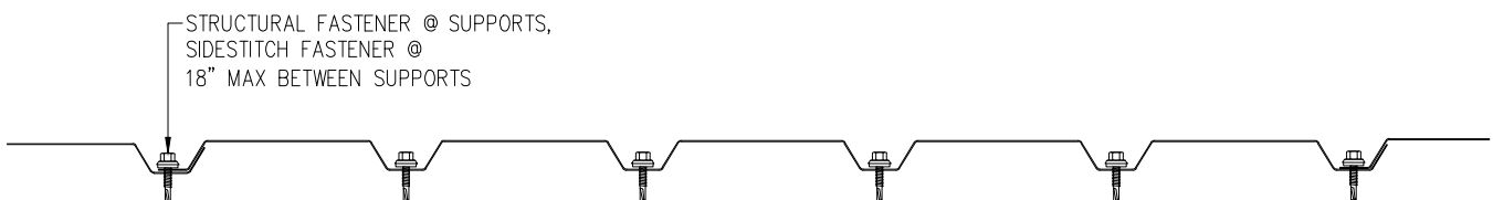
E8-40-W FASTENING PATTERN PROFILE B
