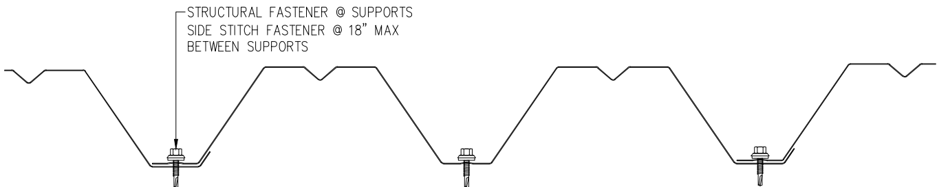
O-24-W FASTENING PATTERN PROFILE B
