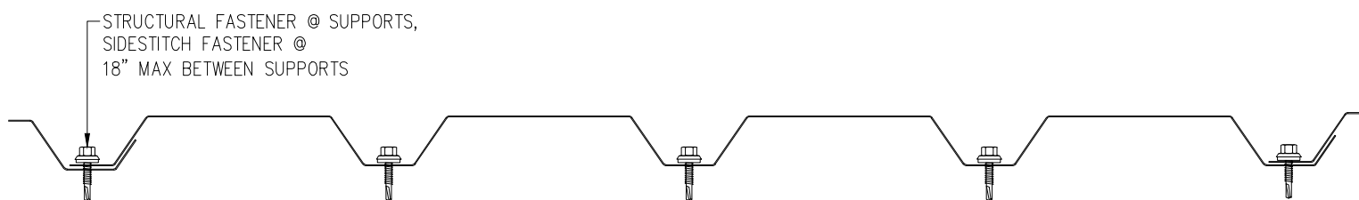
BR9-36-W FASTENING PATTERN PROFILE B
