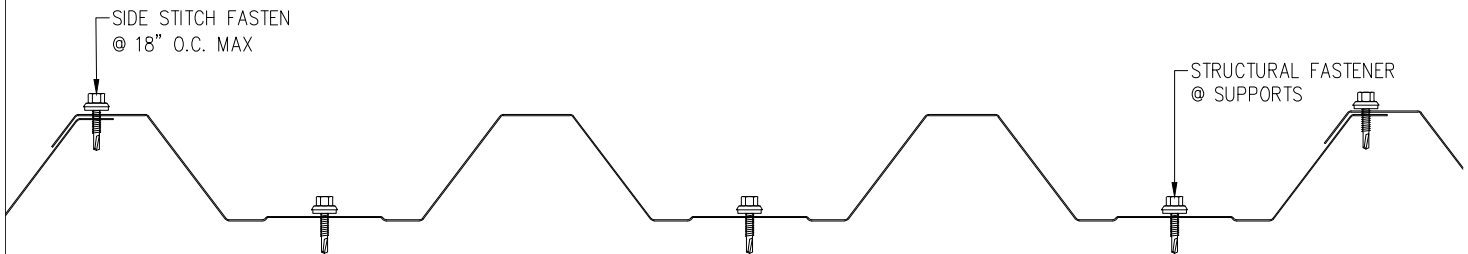
MR-36-EW FASTENING PATTERN PROFILE A
