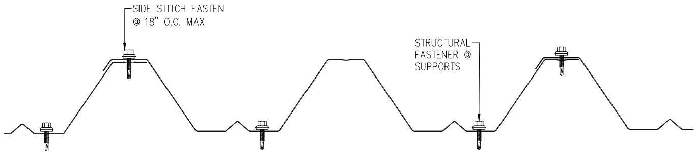
O-24-W FASTENING PATTERN PROFILE A
