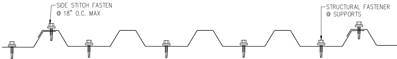
BR-28-ES FASTENING PATTERN PROFILE A
