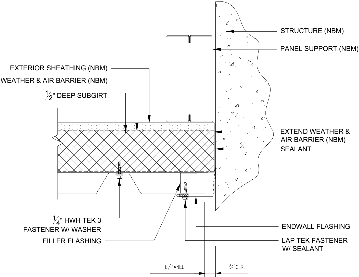
ENDWALL DETAIL
