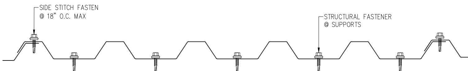
BR7-35-W FASTENING PATTERN PROFILE A
