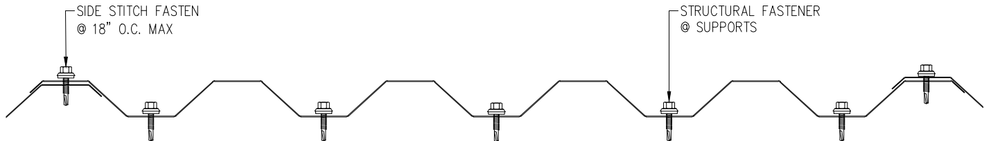
Y-36-ES FASTENING PATTERN PROFILE A
