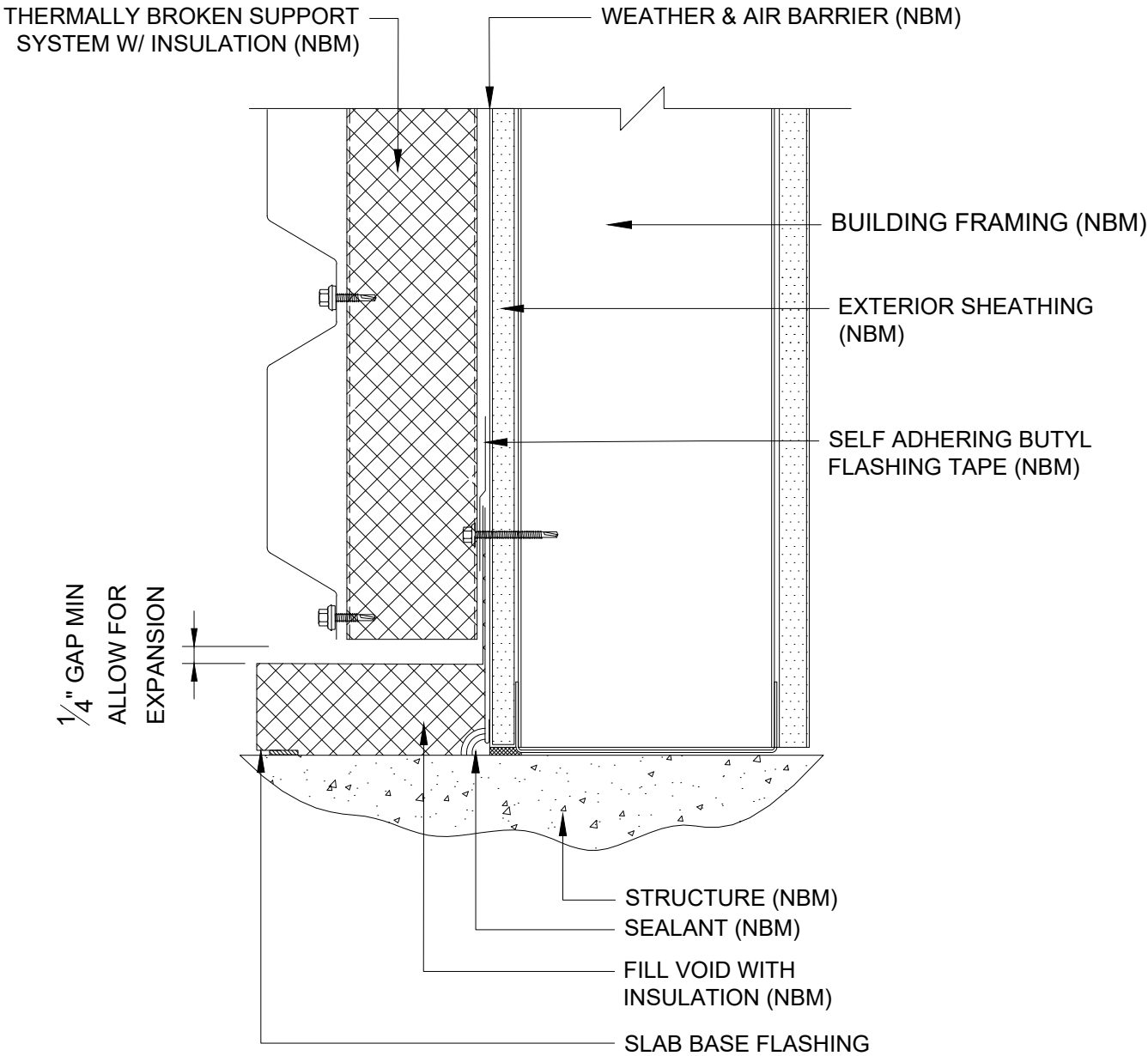
BASE AT SLAB DETAIL
