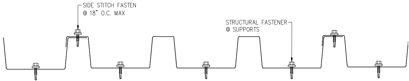
U-24-W FASTENING PATTERN PROFILE A
