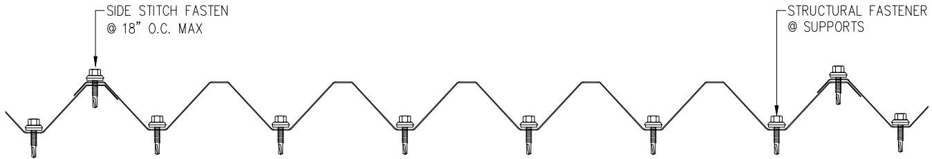
VB-31-S FASTENING PATTERN PROFILE A
