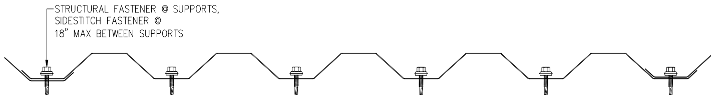
Y-36-ES FASTENING PATTERN PROFILE B
