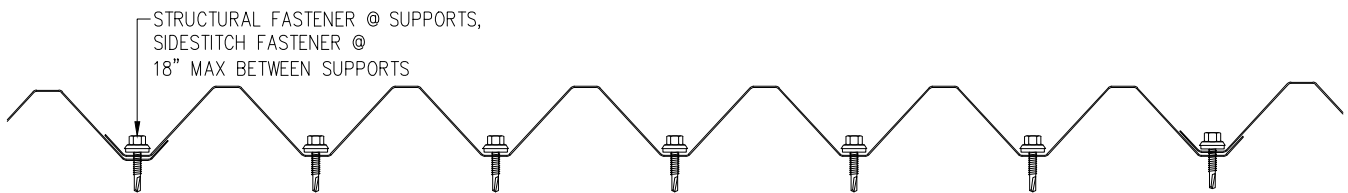
VB-31-S FASTENING PATTERN PROFILE B
