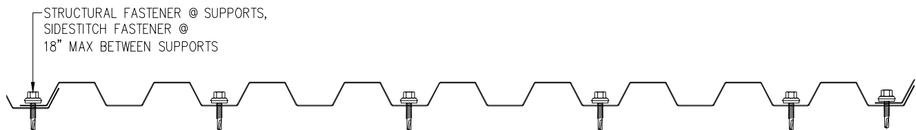
VB-36-W FASTENING PATTERN PROFILE B
