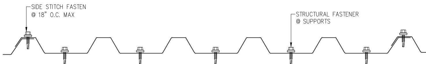
BR-35-S FASTENING PATTERN PROFILE A
