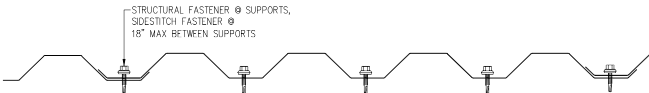
Y-29-ES FASTENING PATTERN PROFILE B
