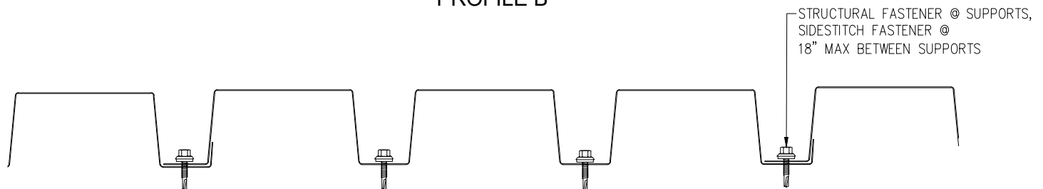
U-24-W FASTENING PATTERN PROFILE B
