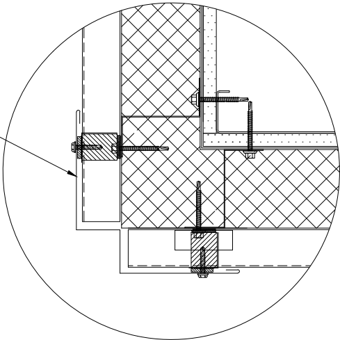
OPTIONAL REVEAL DETAIL
