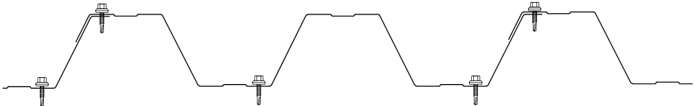
O-24-W FASTENING PATTERN PROFILE A
