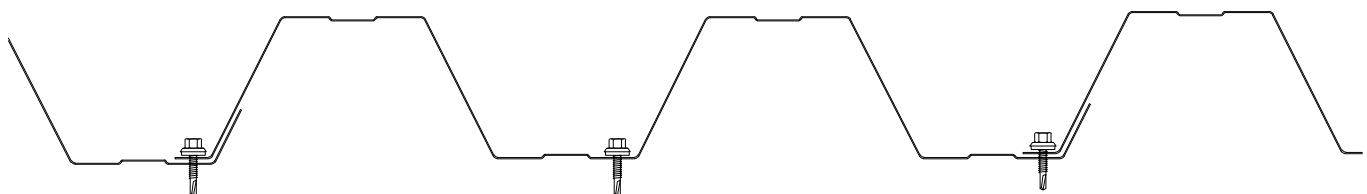
O-24-W FASTENING PATTERN PROFILE B
