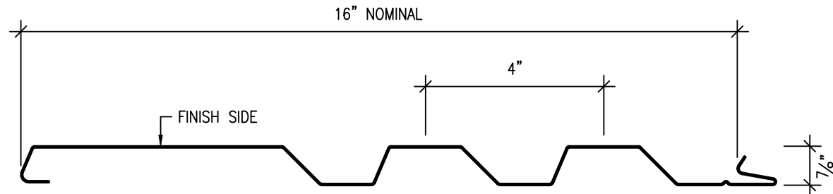
HIGH & LOW CELL DIMENSIONS
