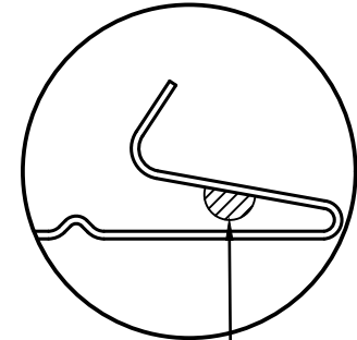
OPTIONAL FACTORY SEALANT (BUTYL PLACEMENT)
