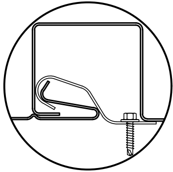
CLIP ENGAGEMENT
