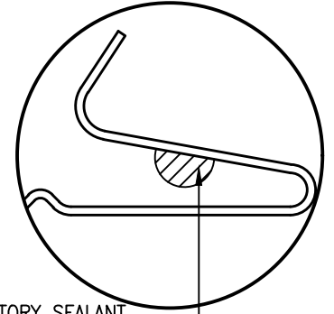
OPTIONAL FACTORY SEALANT (BUTYL PLACEMENT)
