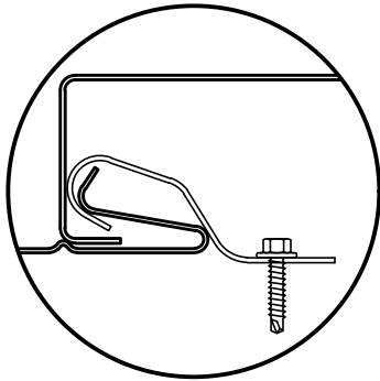
CLIP ENGAGEMENT
