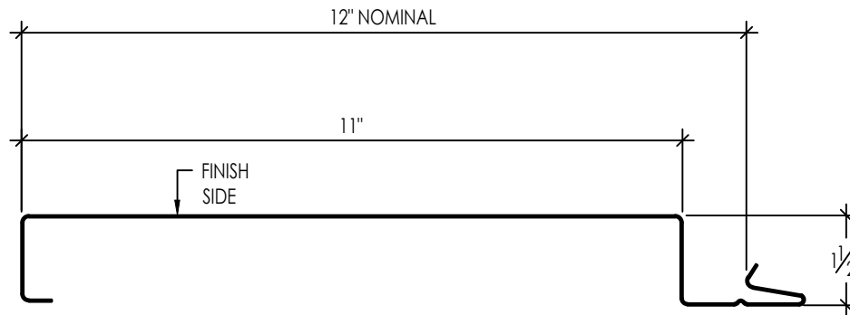
OPTIONAL FACTORY SEALANT (BUTYL PLACEMENT)
