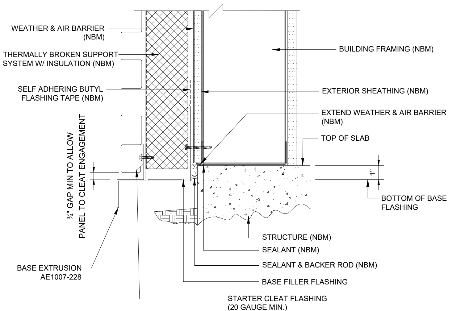
BASE AT CURB OR EDGE OF SLAB EXTRUSION DETAIL
