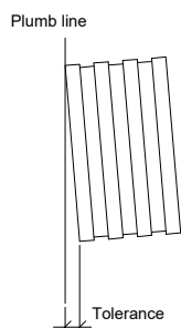
PANEL/ TRIM PLUMBNESS
