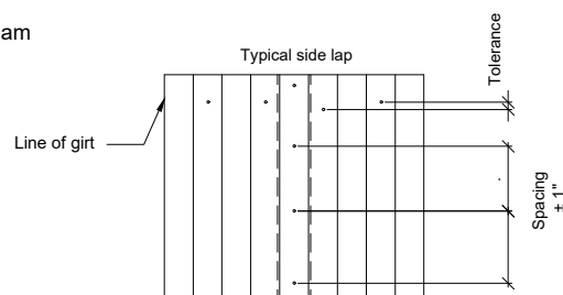
EXPOSED FASTENER
