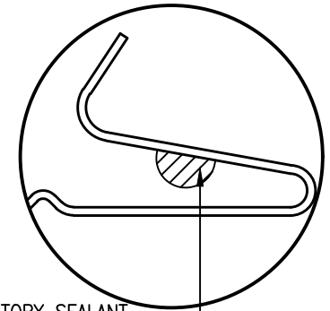
OPTIONAL FACTORY SEALANT (BUTYL PLACEMENT)
