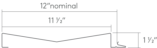
Panel Profile
