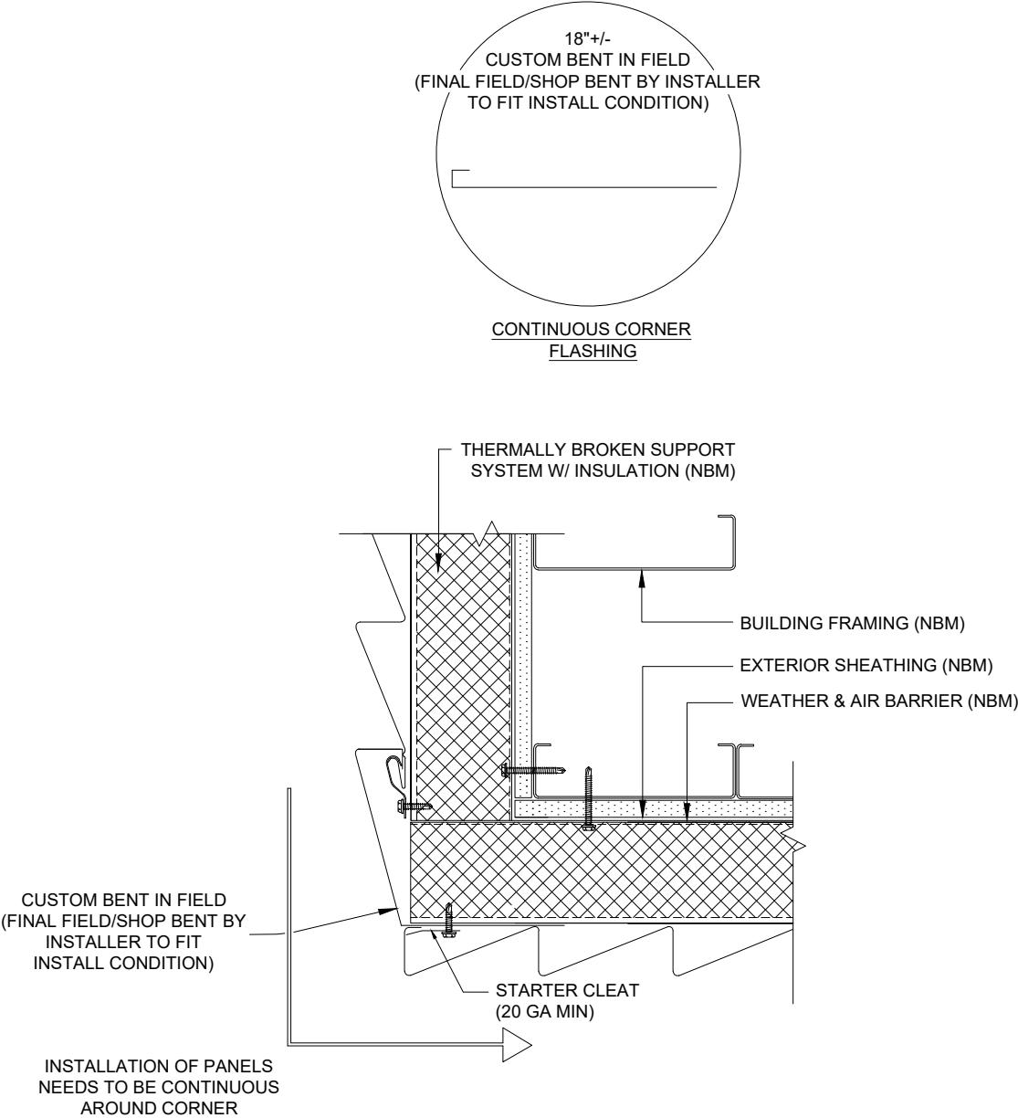
CONTINUOUS CORNER DETAIL
