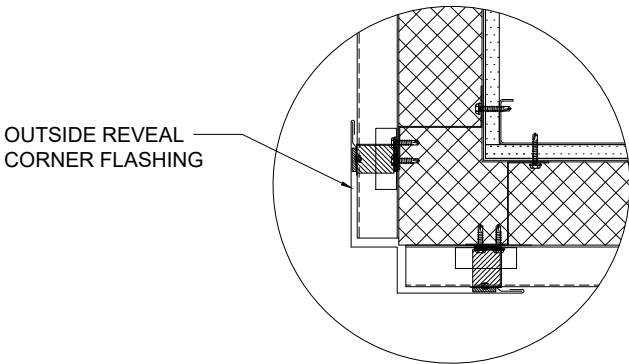
OPTIONAL REVEAL DETAIL
