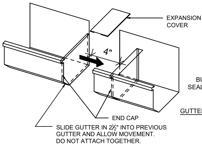
GUTTER EXPANSION DETAIL
