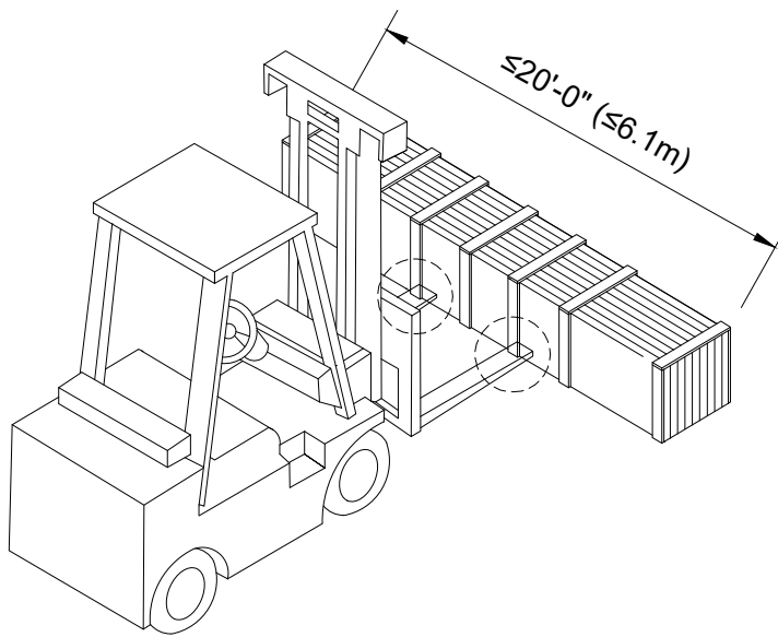
FIG.1 PREFERRED METHOD (1 FORKLIFT)
