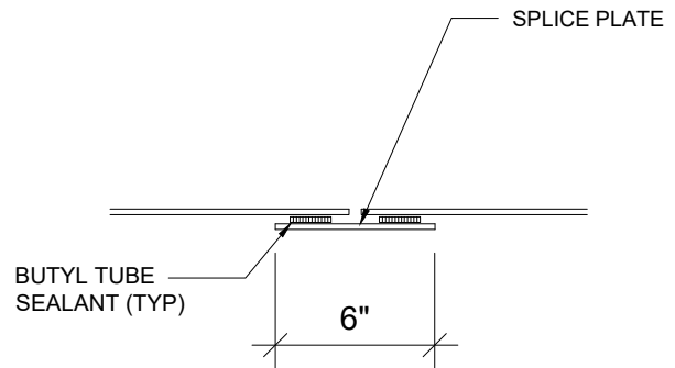
RAKE LAP DETAIL
