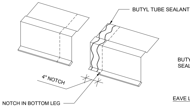
EAVE INSIDE SPLICE PLATE
