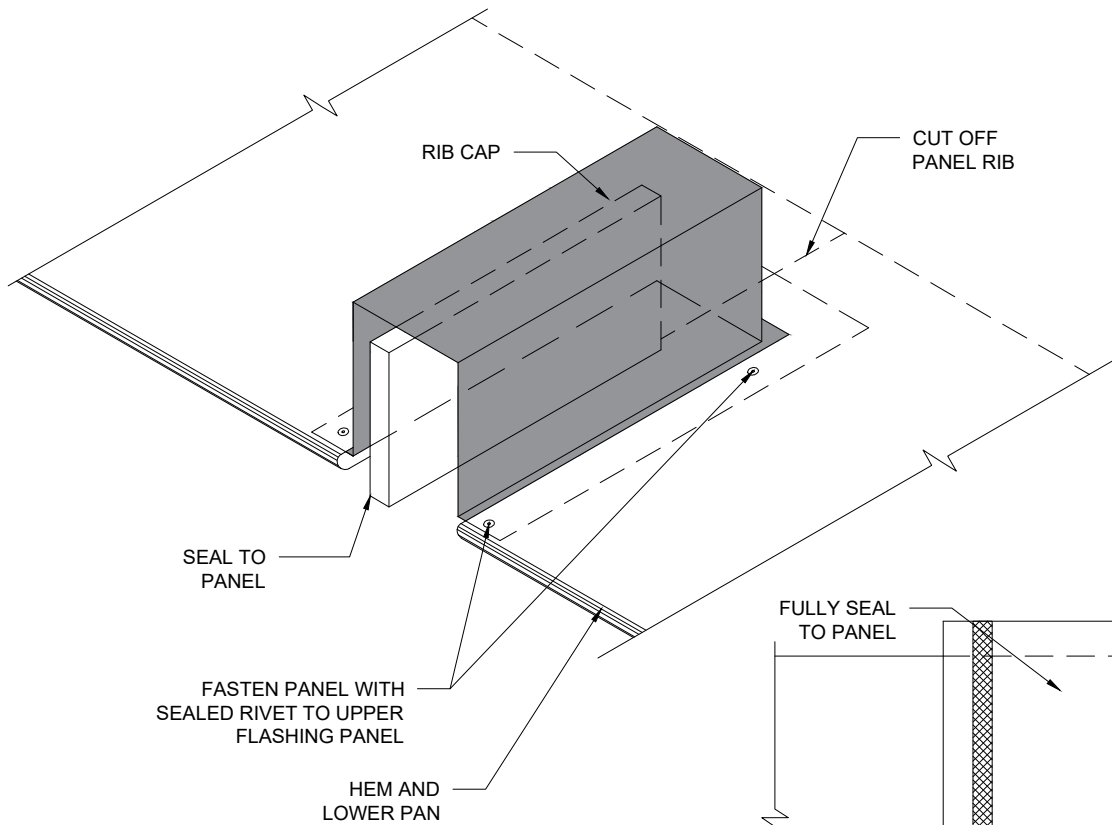
RIB CAP DETAIL
