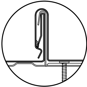
CLIP ENGAGEMENT
