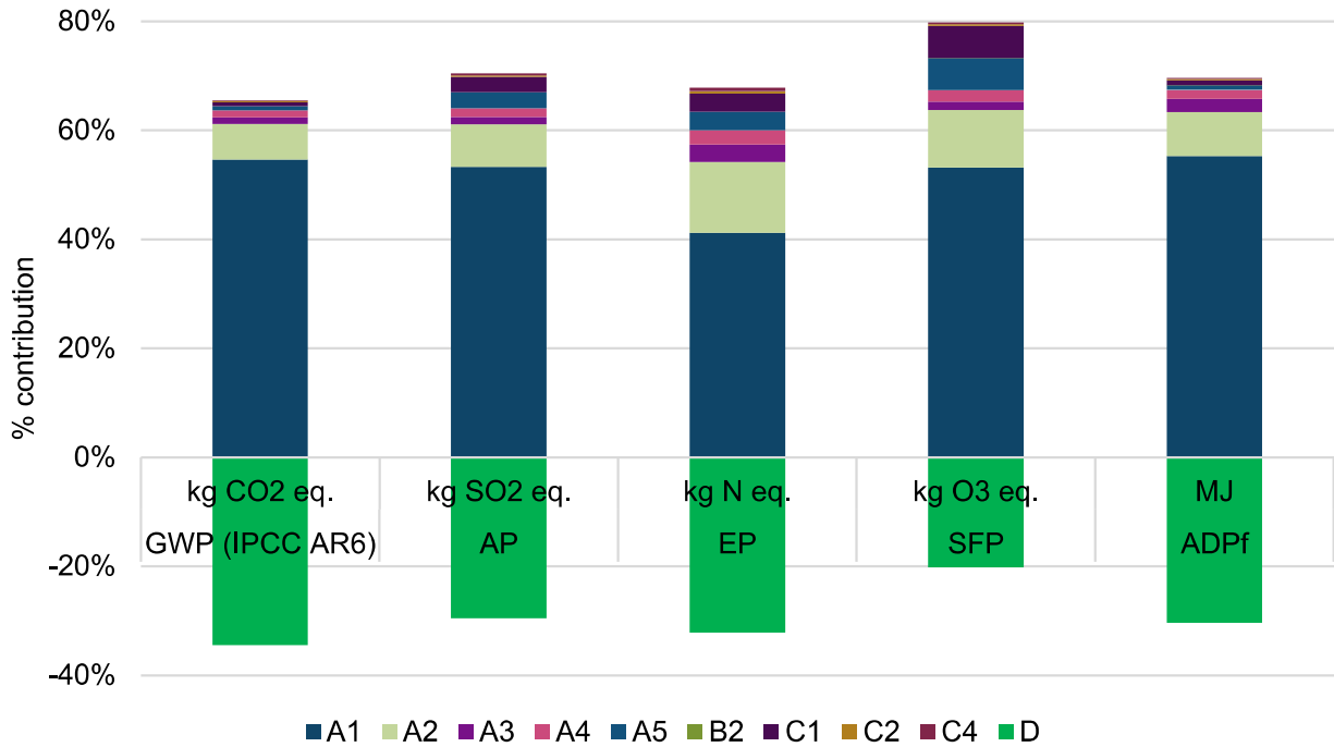
Figure 3. Contribution Analysis for weighted average LCIA results – Steel Cladding (100m² installed)
